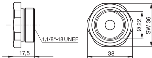
Sight glass type GSG-22-17,5
