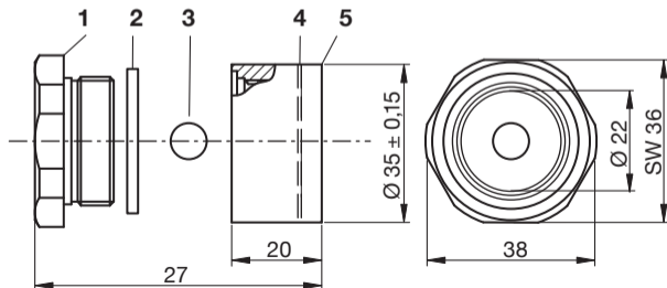
Sight glass set type SSG-22G
