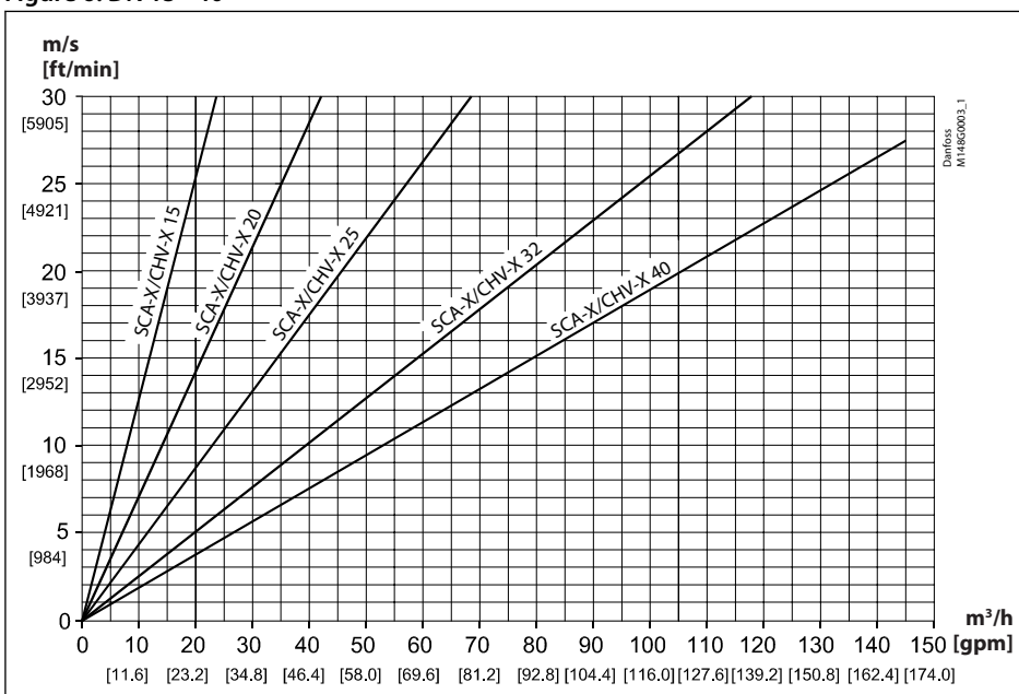
Figure 6: DN 15 - 40
